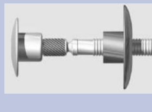
HUCKTAINER & COLLAR TO FIT HANDLE HUB
